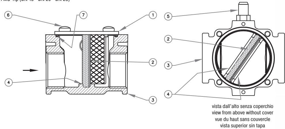
fig. 1 FMC Rp (DN 15 - DN 20 - DN 25)
